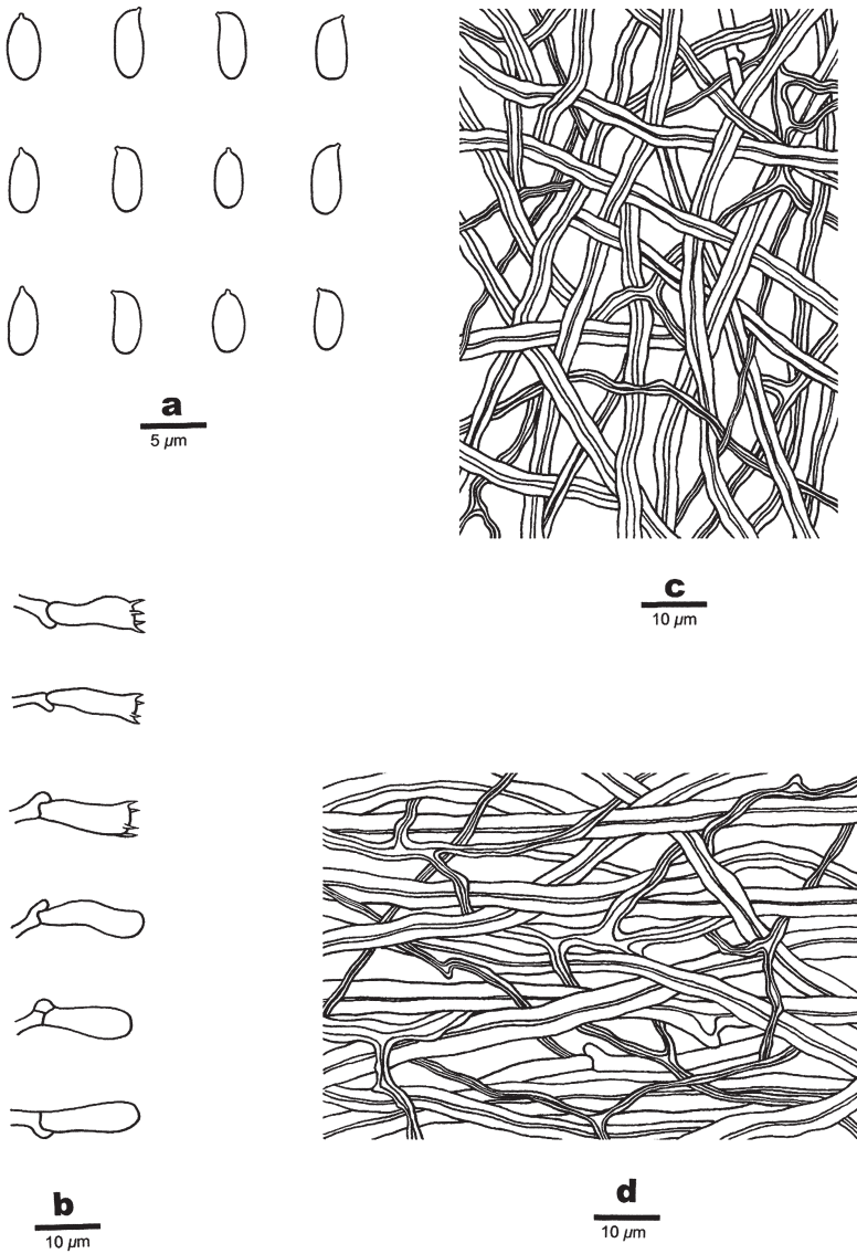
FIG. 2. Microscopic structures of Trametes maxima (drawn from Dai 6865). a: Basidiospores. b: Basidia and basidioles. c: Hyphae from tube. d: Hyphae from context.
