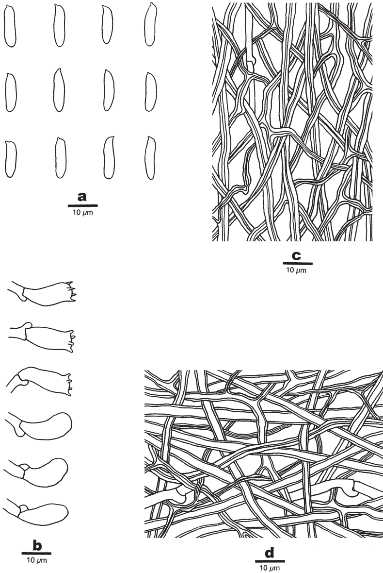
FIG. 3. Microscopic structures of Trametes mimites (drawn from Dai 10608). a: Basidiospores. b: Basidia and basidioles. c: Hyphae from tube. d: Hyphae from context.
