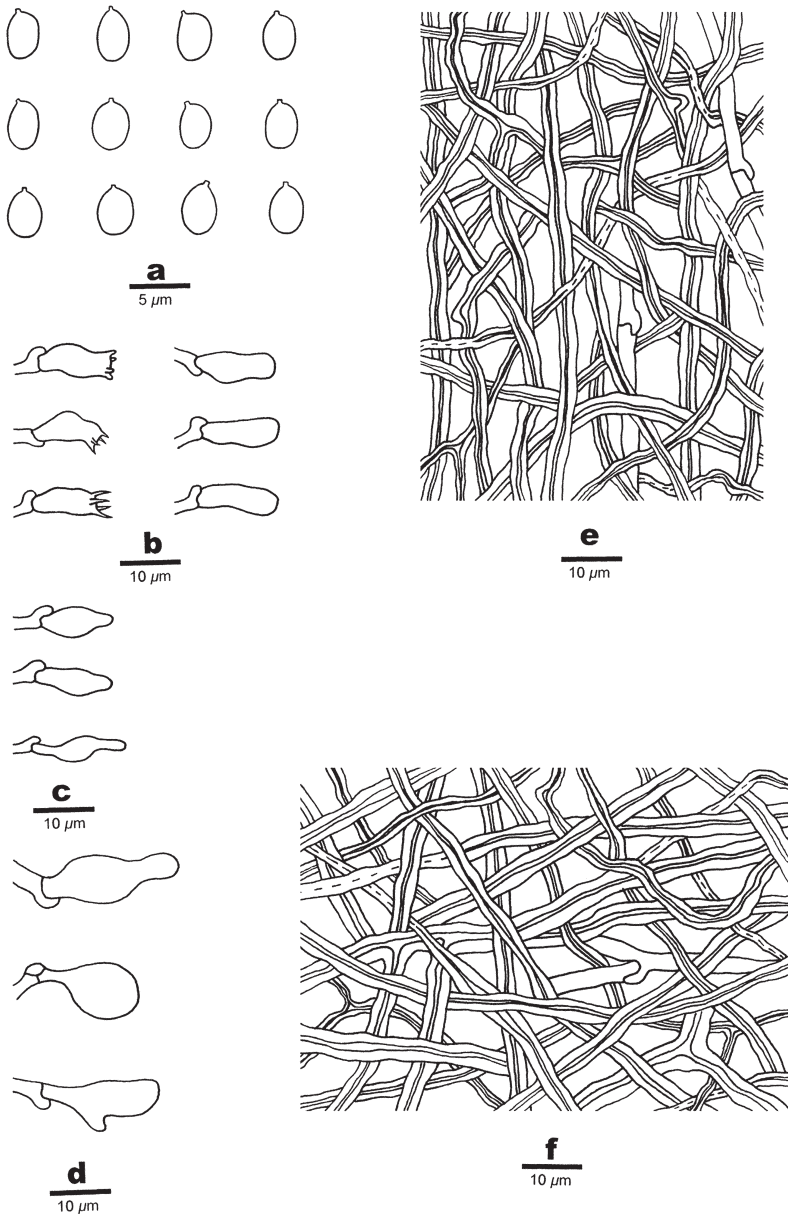
FIG. 1. Microscopic structures of Trametes ellipsospora (drawn from Cui 6259).
