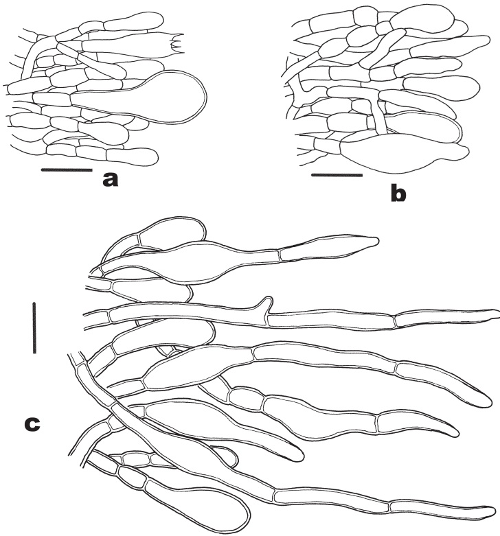
FIG. 3. Stipitipellis of Phylloporus luxiensis (HKAS 57036). a. From the apex of the stipe. b. From the middle part of the stipe. c. From the basal part of the stipe. Bars= 20 \mu\text{m} .
