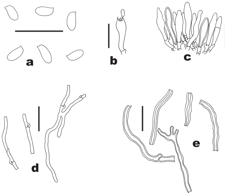
FIG. 5. Microscopic features of Phylloporus scabrosus (HKAS 28981, holotype). a. Basidiospores. b. Basidium. c. Cystidia. d. Generative hyphae. e. Skeletal hyphae. Bars = 20 \mu\text{m} .
