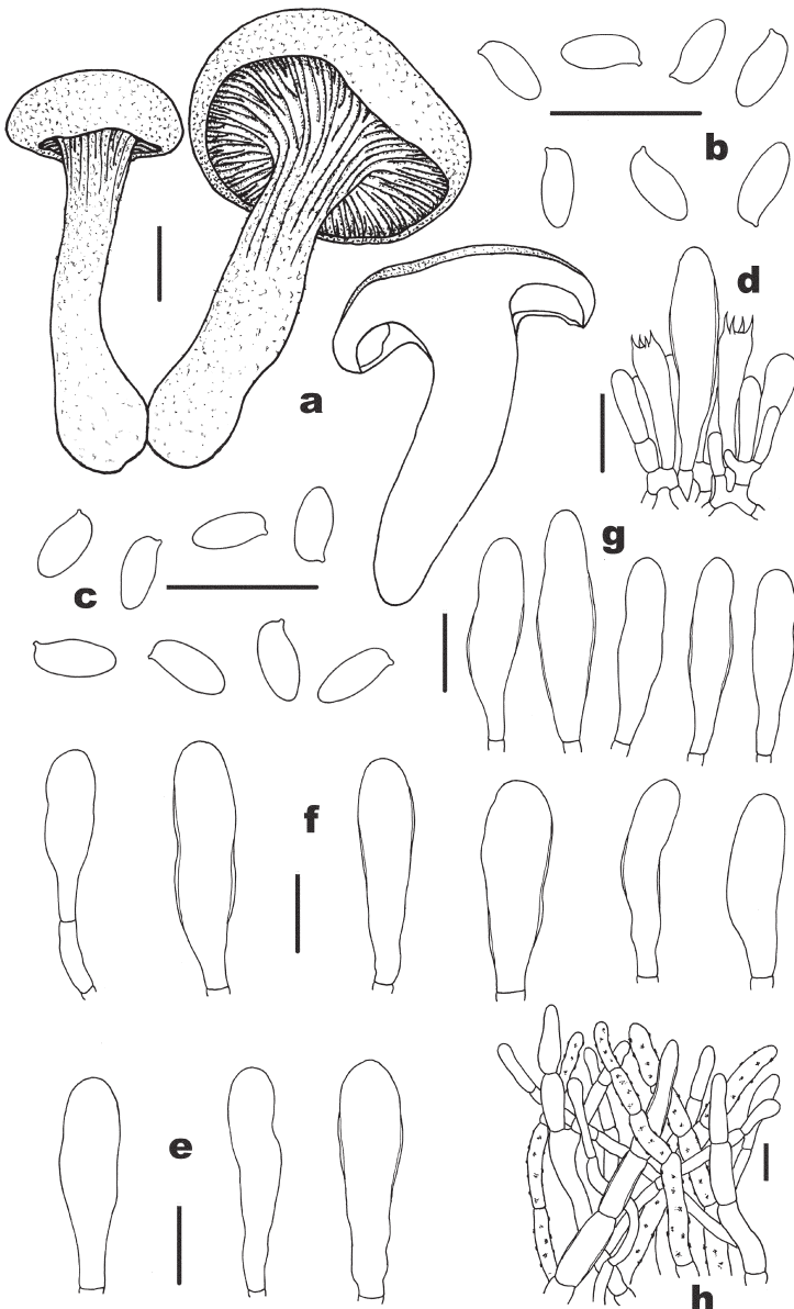
FIG. 2. Macroscopic and microscopic features of Phylloporus luxiensis (a from HKAS 57048; b, e from HKAS 40150, holotype; c–d, f–h from HKAS 57036). a. Basidiomata. b–c. Basidiospores. d. Basidia and pleurocystidium. e. Pleurocystidia. f. Cheilocystidia. g. Pleurocystidia. h. Pileipellis. Bars: a = 2 cm; b–h = 20 \mu m.
