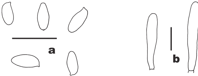
FIG. 4. Microscopic features of Phylloporus sulcatus (FH 3725, holotype). a. Basidiospores. b. Pleurocystidia. Bars = 20 \mu m.
