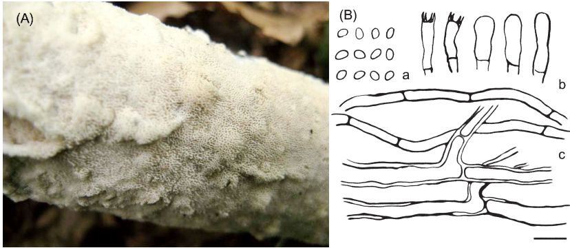
FIG. 1. Ceriporia lacerata . (A) Basidiocarp. (B) Microscopic features: a, basidiospores; b, basidia; c, generative hyphae. Scale bar = 10µm
